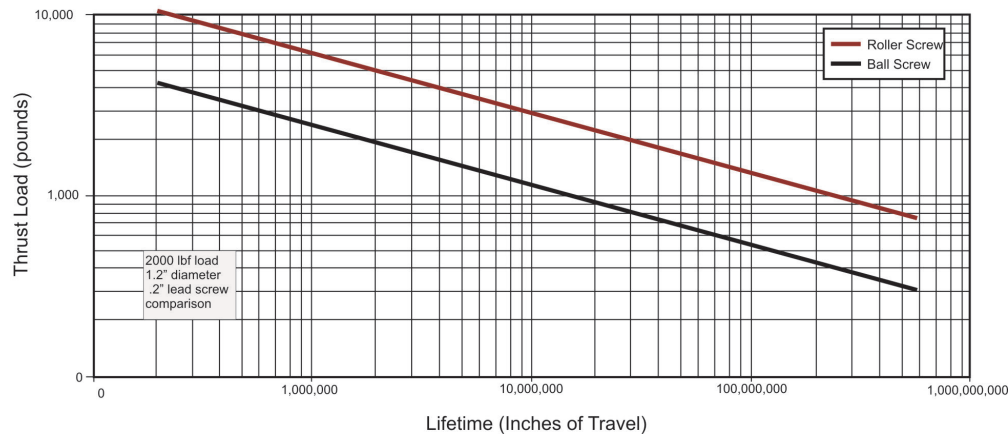
Lifetime Comparison (Roller vs Ball Screws)
